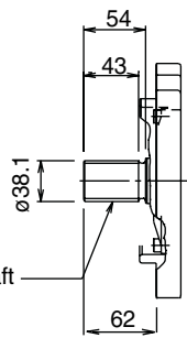
Shaft Detail – SAE "CC" Spline
