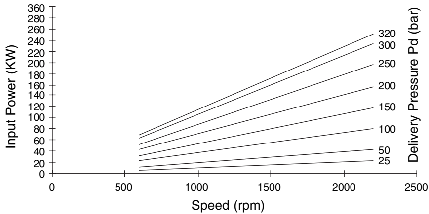
K3VL200 Theoretical Power Curve
